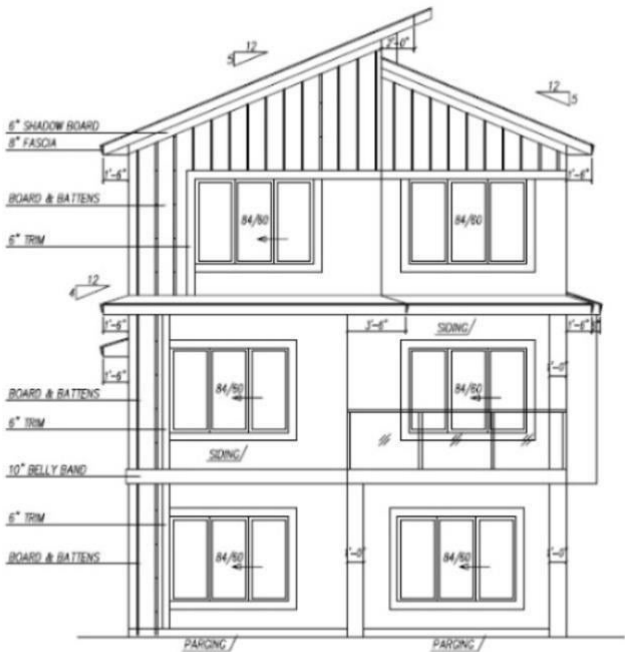
REAR ELEVATION
